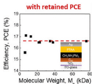
Flexible Solar Cell incorporating PTAA
